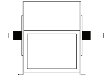
Arrangement 6 Double inlet bearer bar
