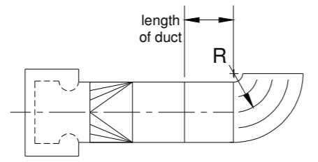
b) Square elbow with inlet transition – three long turning vanes
