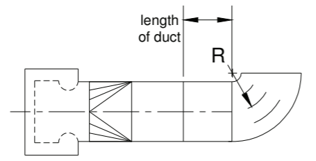
c) Square elbow with inlet transition – short turning vanes
