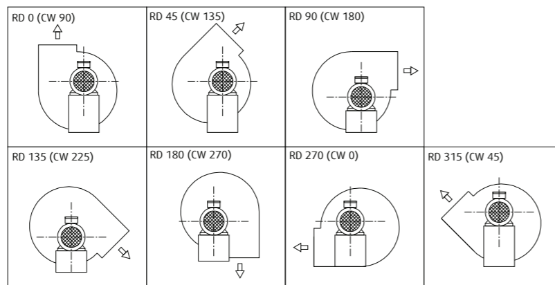
Standard discharge positions for centrifugal fans
