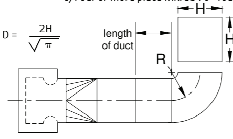
a) Square elbow with inlet transition – no turning vanes
